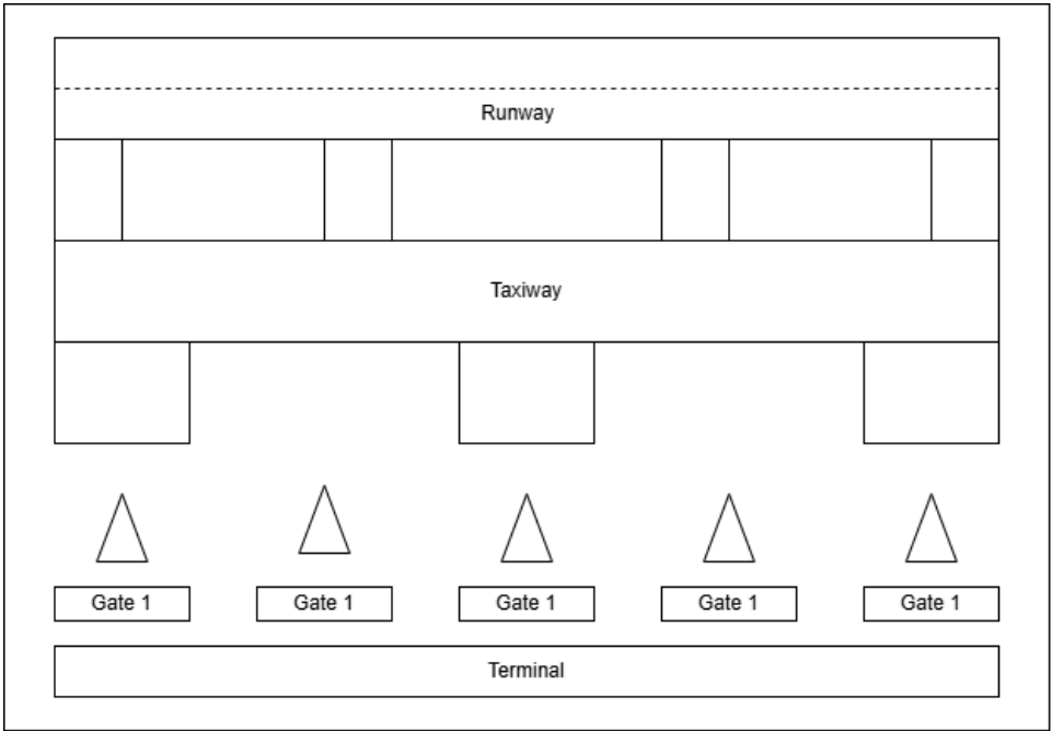
UML design
